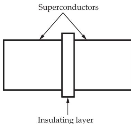
Fig. Q.29.1 Josephson junction
