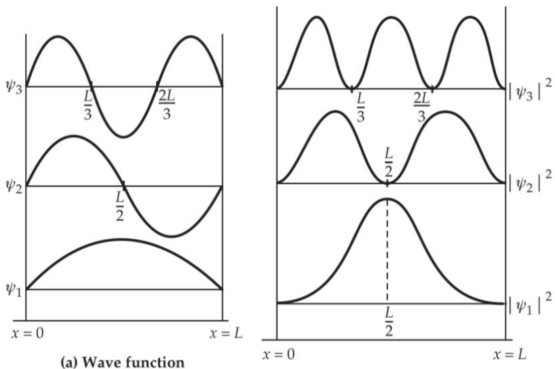
(b) Probability function
